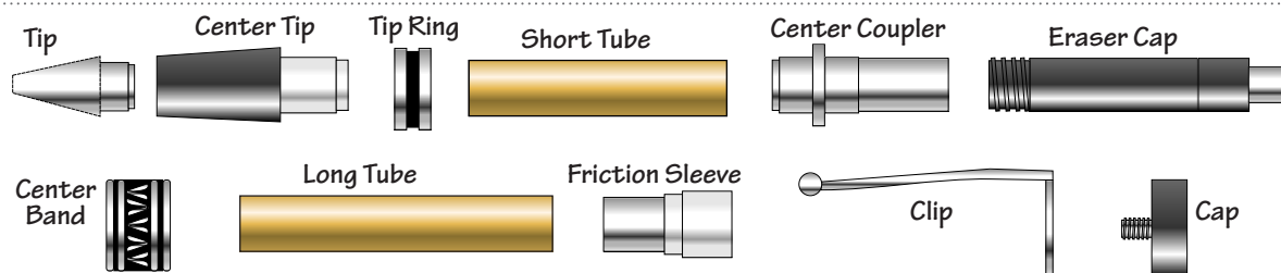
Pencil Transmission (.7mm lead)
